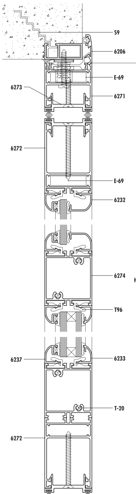
PVVC Corte 6-7-8
