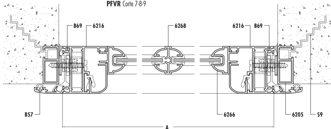
PFVR Corte 7-8-9
