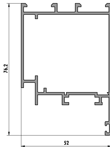
6214 (1,088 kg/m)
