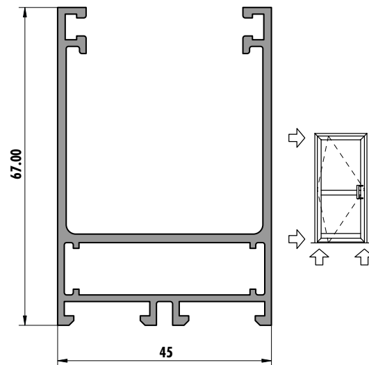
6272 (1,156 kg/m)
