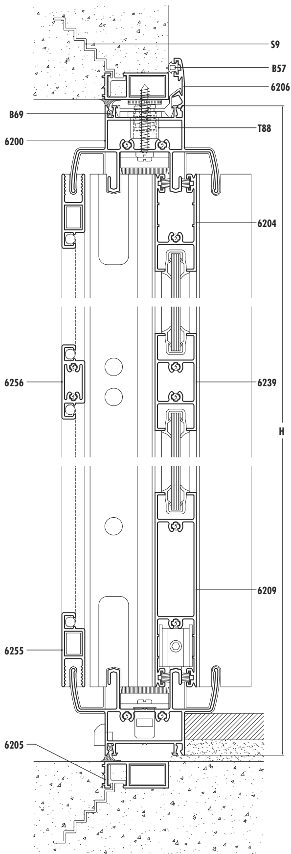
PC Corte 6-7-8
