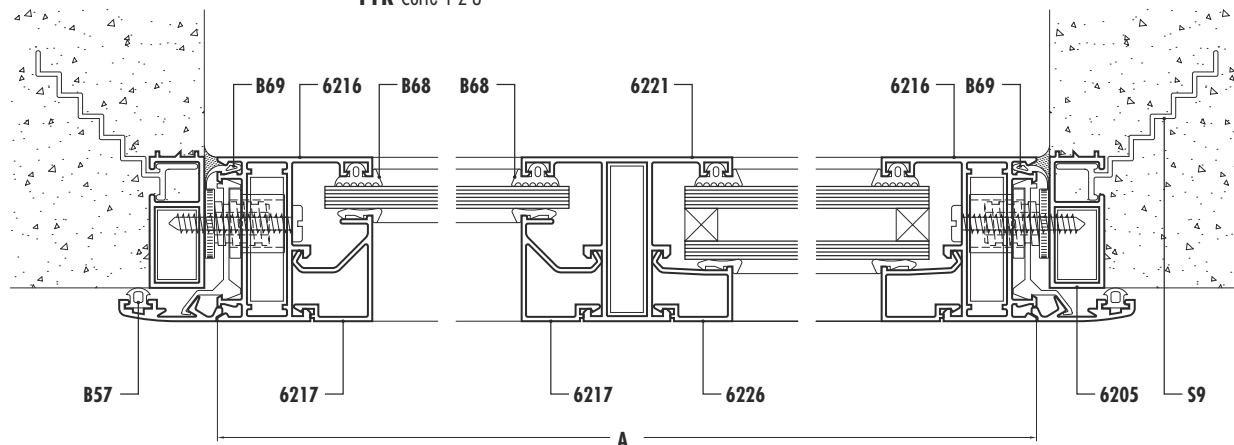
PFR Corte 1-2-3
