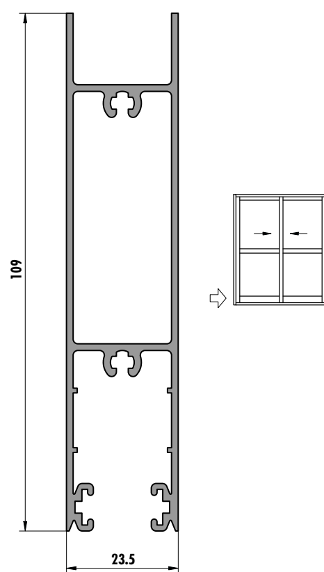
6252 (1,215 kg/m)
