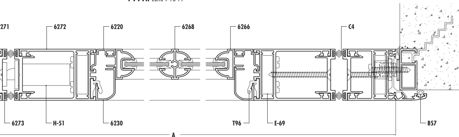
PVVVR Corte 9-10-11
