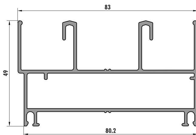
6905 (1,318 Kg/m)
