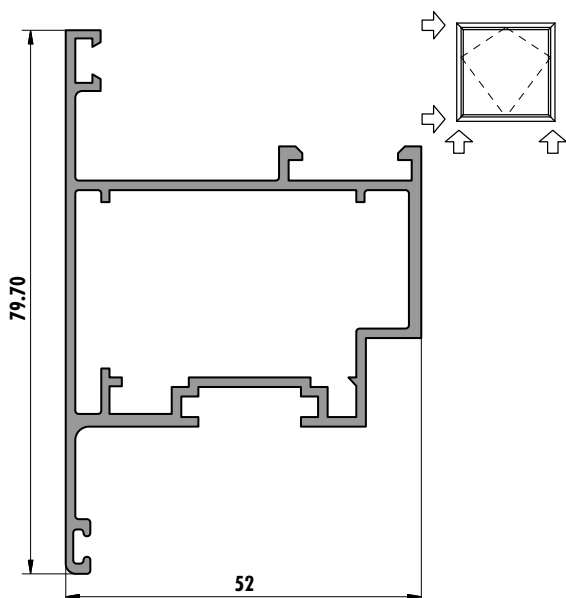
6258 (1,061 kg/m)
