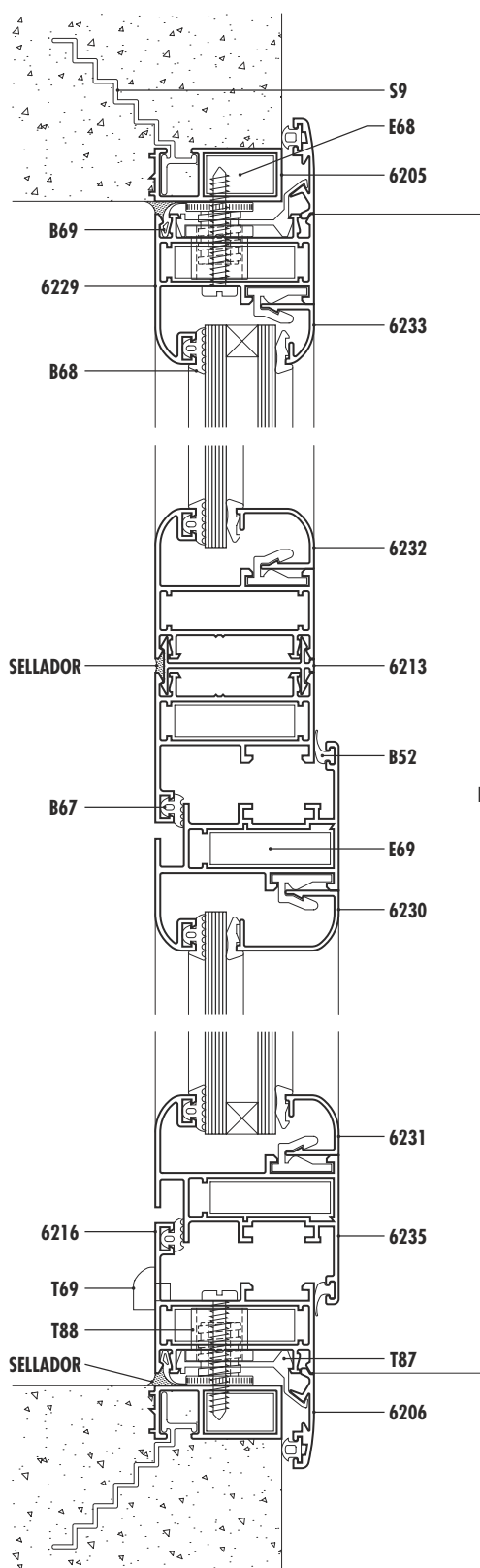
VADCC / PF Corte 6-7-8
