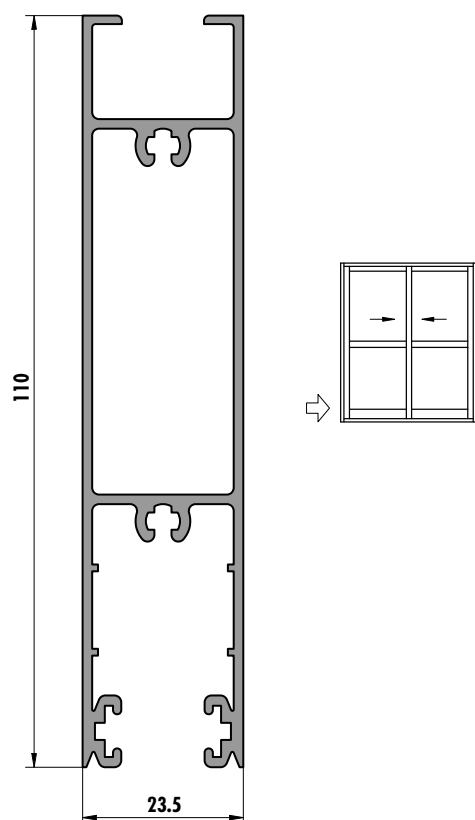
6209 (1,258 kg/m)
