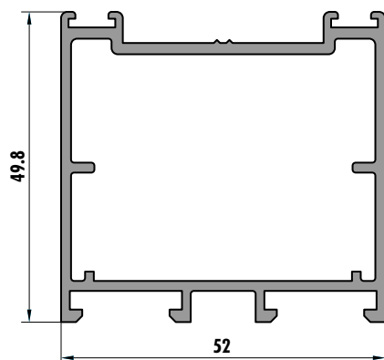
6285 (1,040 kg/m)
