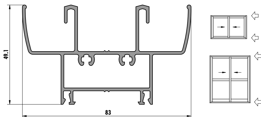
6200 (1,266 kg/m)
