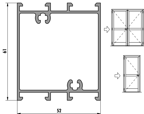
6218 (1,150 kg/m)
