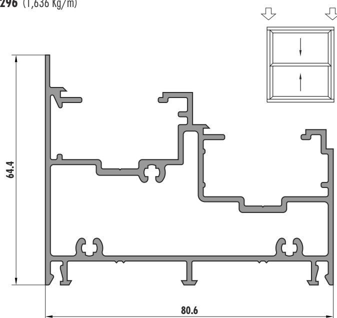
6296 (1,636 Kg/m)
