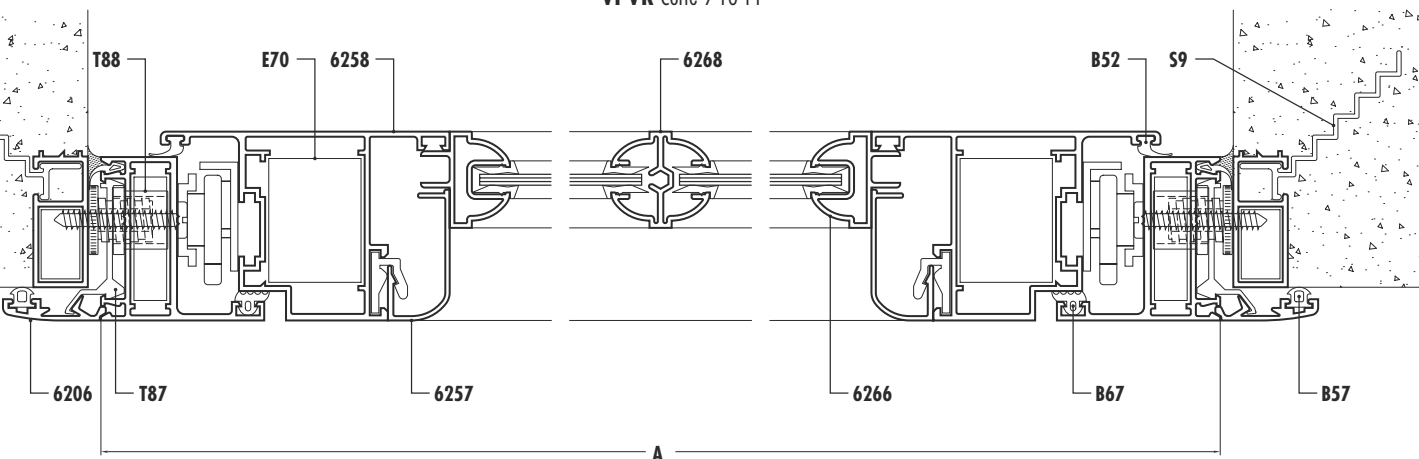
VPVR Corte 9-10-11
