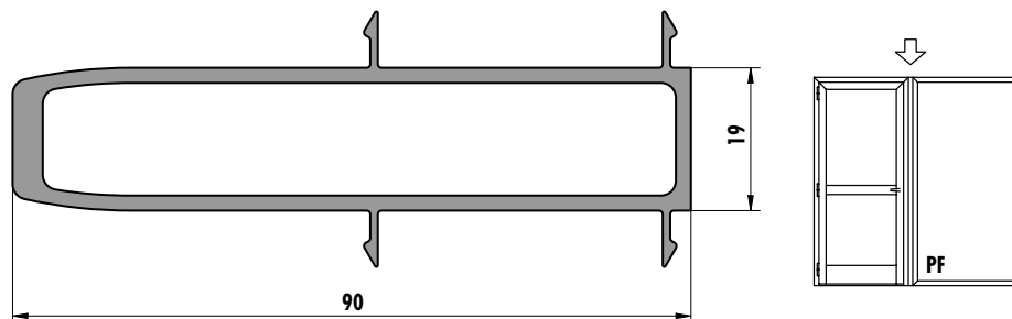
6261 (1,280 kg/m)
