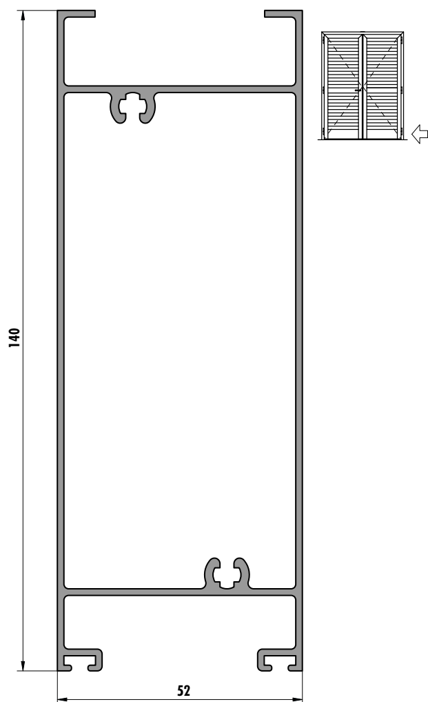
6281 (1,723 kg/m)
