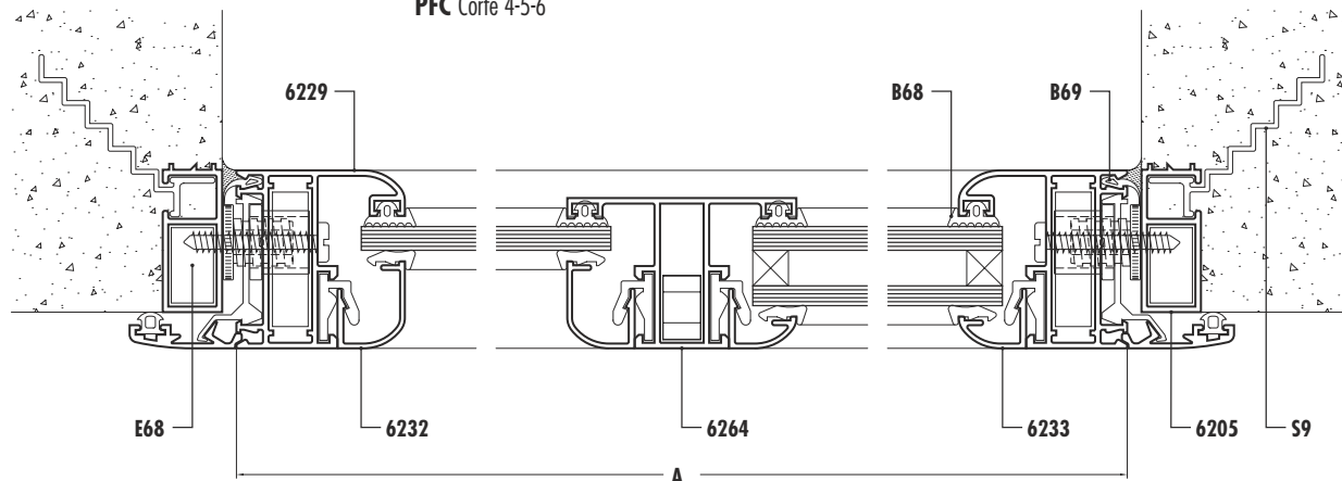
PFC Corte 4-5-6
