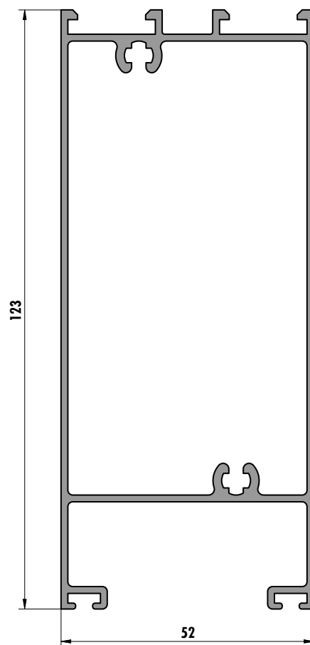
6219 (1,647 kg/m)
