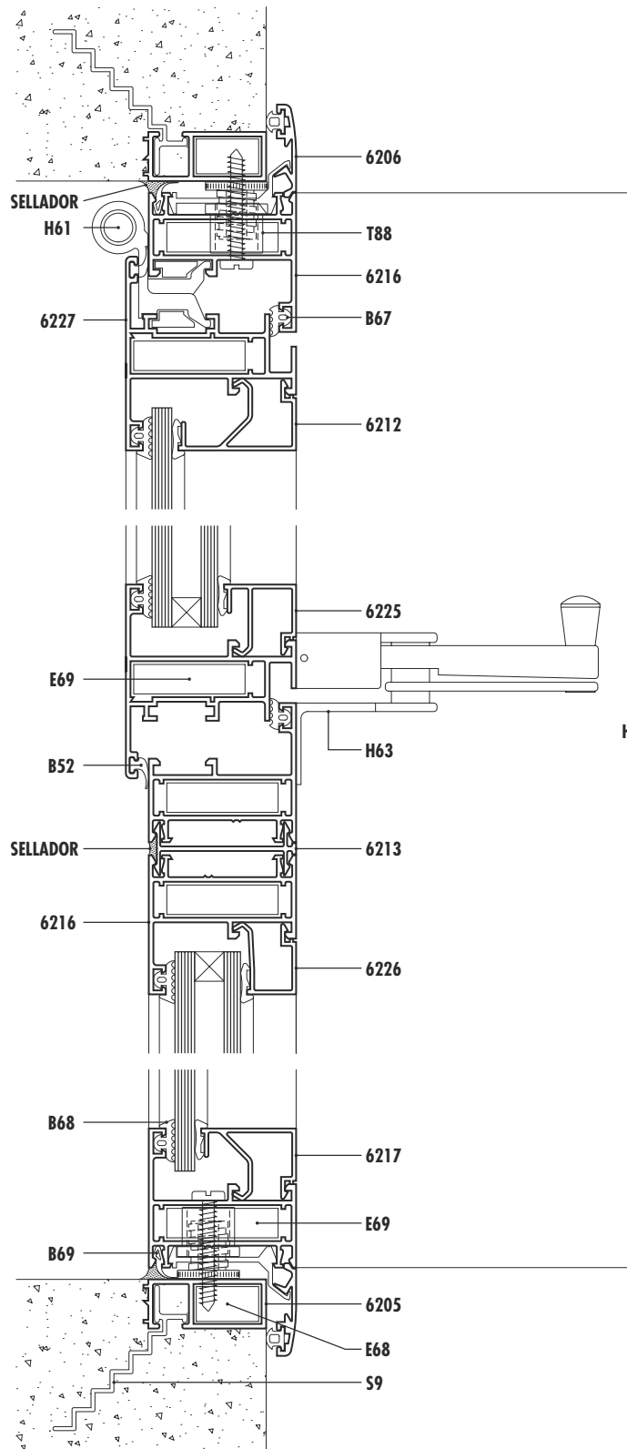
VVR / PF Corte 6-7-8
