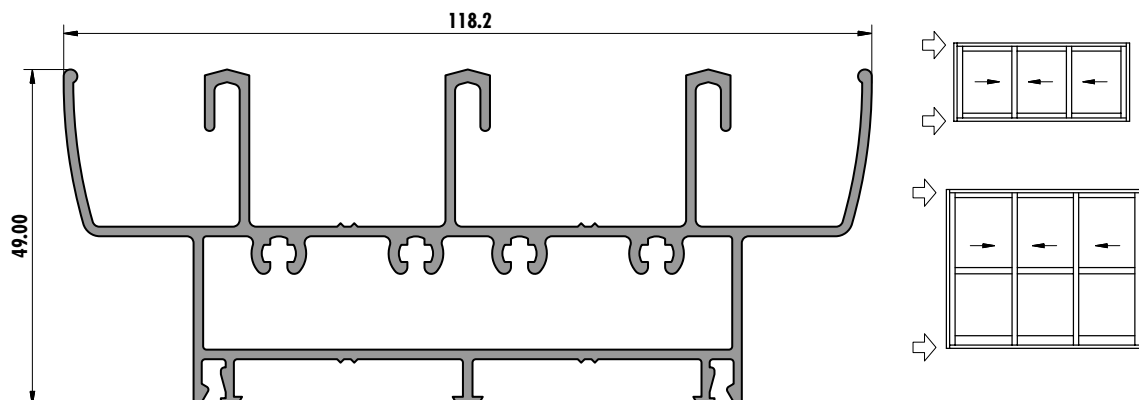
6240 (1,823 kg/m)
