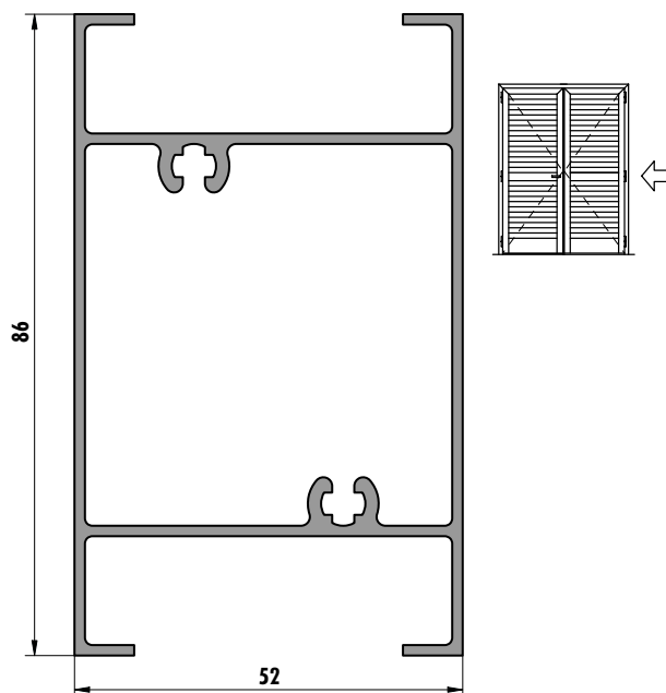
6276 (1,315 kg/m)
