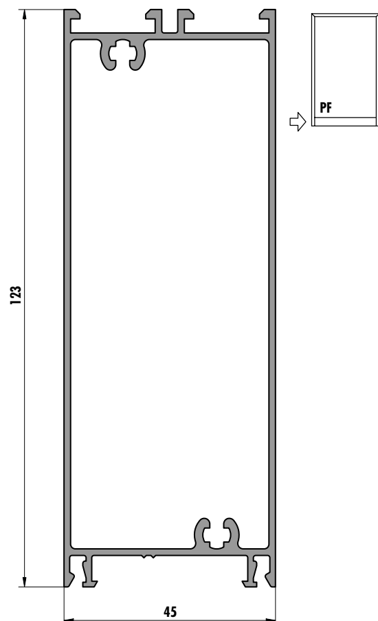
6263 (1,671 kg/m)
